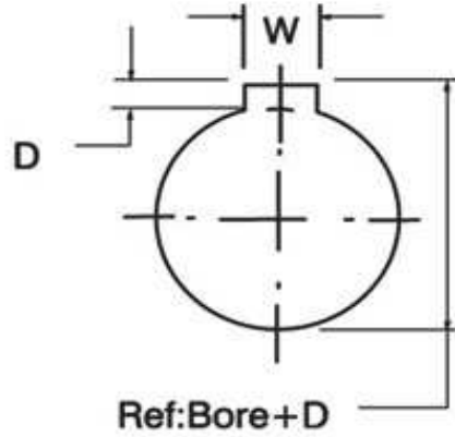
MM Bore Key way dimensions conform to ISO standard Depth measured at centerline.
